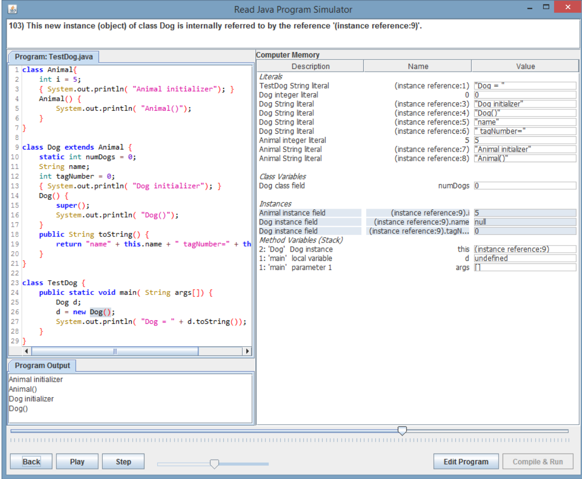
Figure 12: Class instantiation example showing class variable and instance fields in the process of be allocated and initialized.
